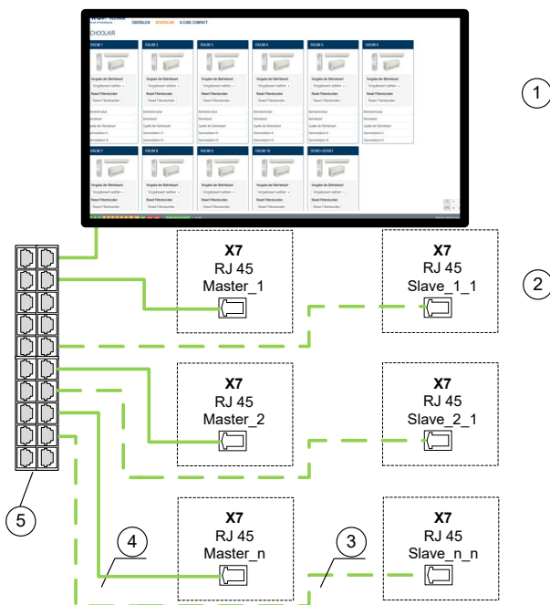
Abb. 19: FSL-CONTROL III X-TAIRMINAL (1)
