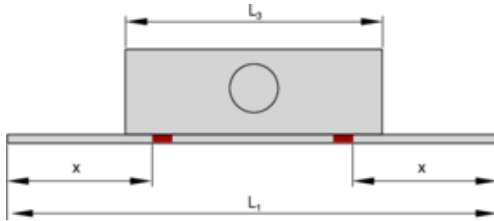
Fig. 15: Front rail longer than plenum box, centre position of plenum box, X = (L_1 - L_2) / 2 + 45
