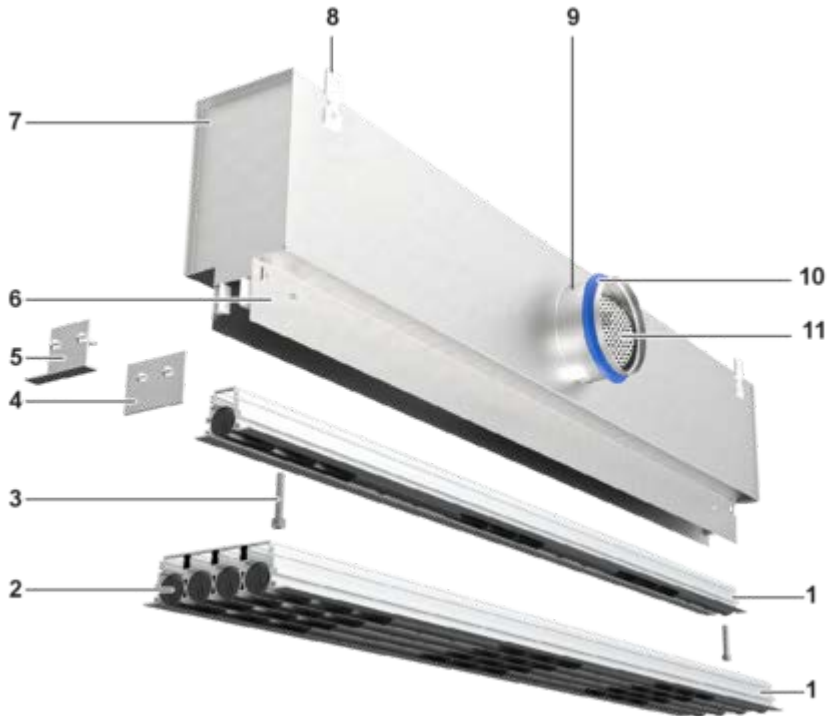
Fig. 1: Schematic illustration example PL35-*-SF
