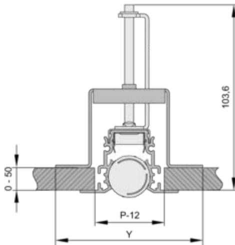
Fig. 17: Position of the crossbar, ceiling thickness up to 50 mm
