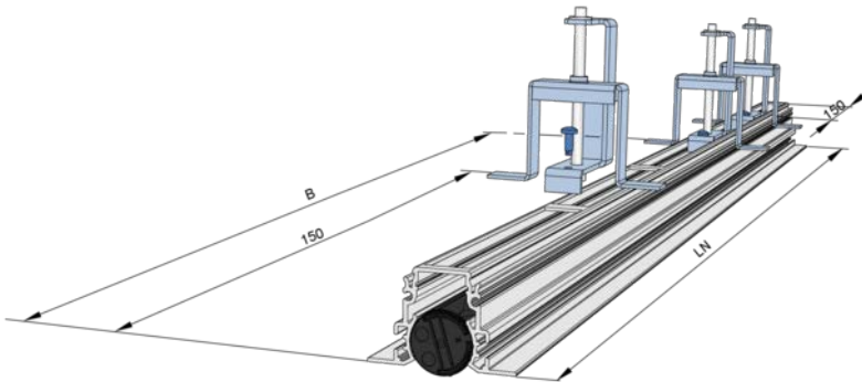
Fig. 20: 3 fixing points from L_N \geq 1500 mm
