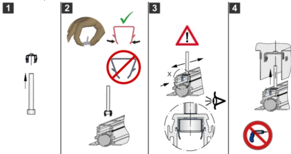
Fig. 11: Front rails with detachable diffuser face fixing
